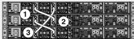
Figure 16. Stack cable connections after switch 4 has been removed from the stack
