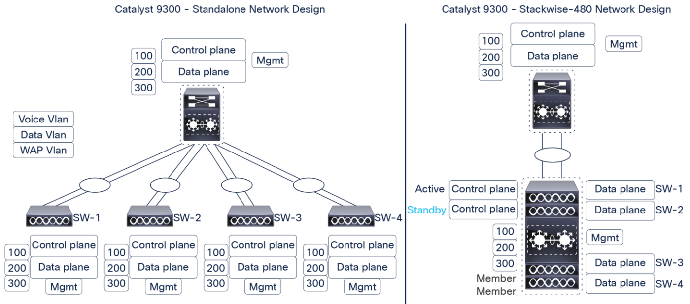
Figure 20. Comparison of Cisco Catalyst 9300 Series Switches in standalone mode to a StackWise-1T/480/320 multilayer
