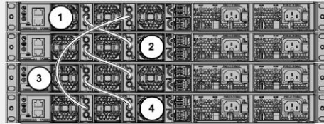
Figure 15. Stack cable connections with four switches in the stack
