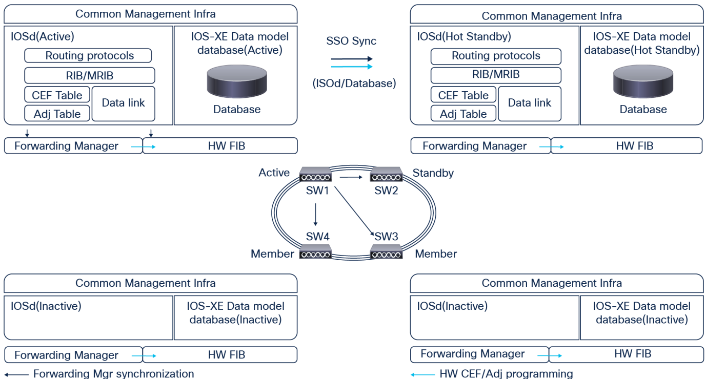
Figure 11. Cisco Catalyst 9300 Series and centralized processing
