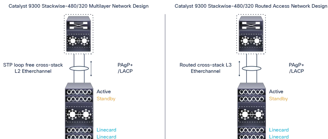
Figure 22. Cisco Catalyst 9300 Series cross-stack EtherChannel design
